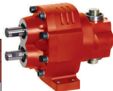
GEAR PUMP WITH SHAFT & PNEUMATIC VALVE BI-DIRECTIONAL
